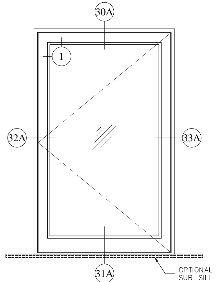
EXTERIOR ELEVATION VIEW
